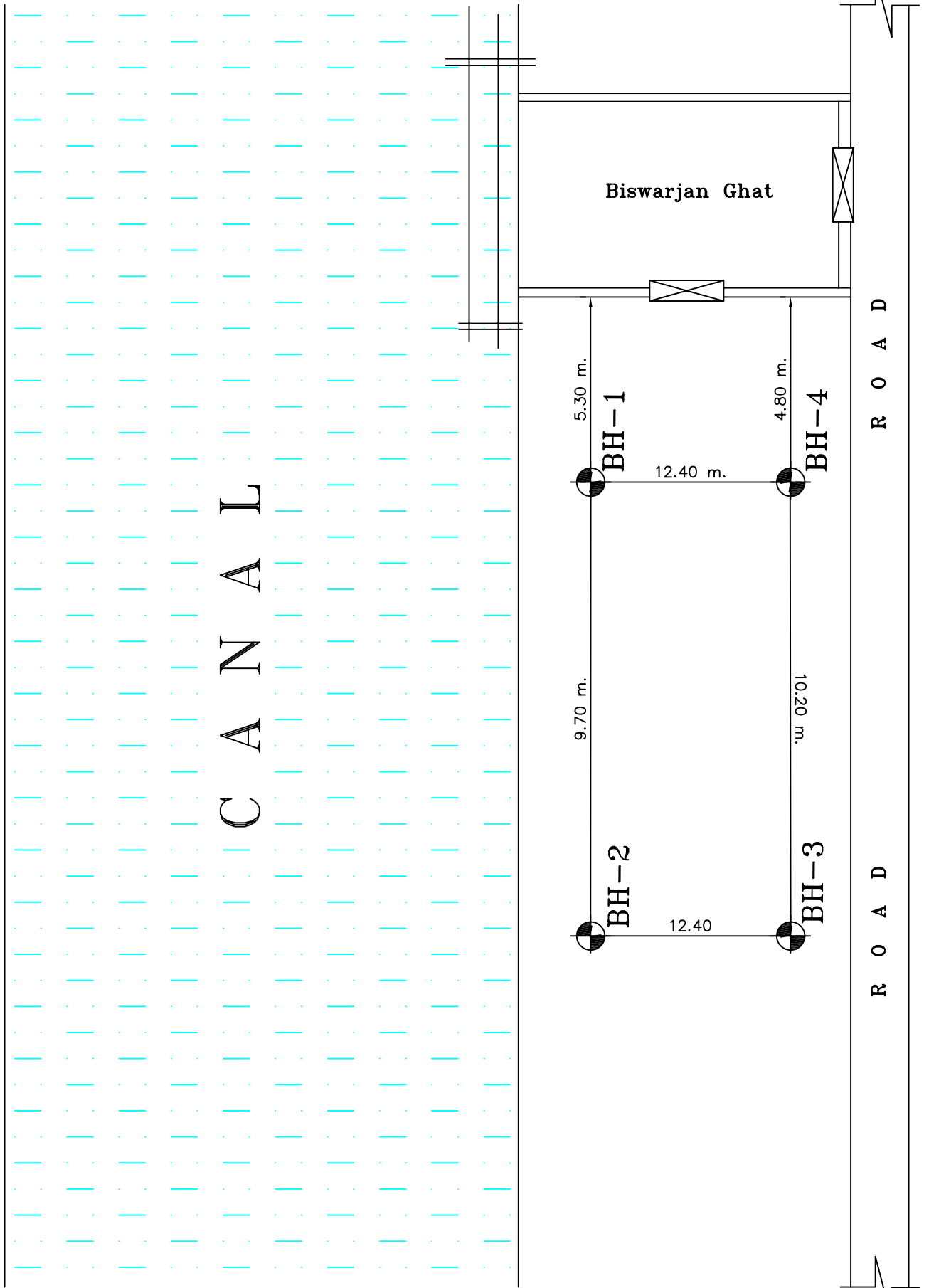
Figure 1 : Site Plan and Location of Boreholes Not To Scale
